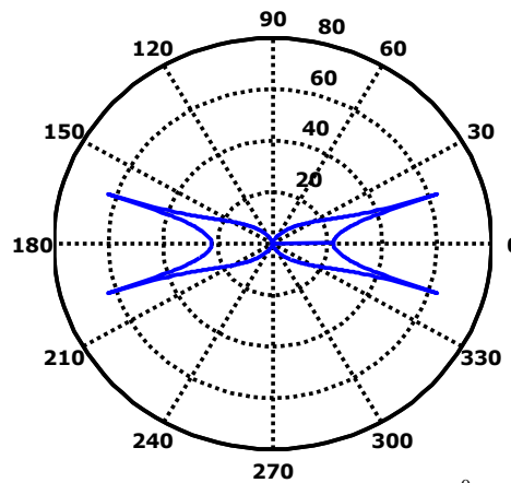
Figure 4: Radiation pattern of rectangular patch antenna in H-plane ( \phi = 0^\circ )
