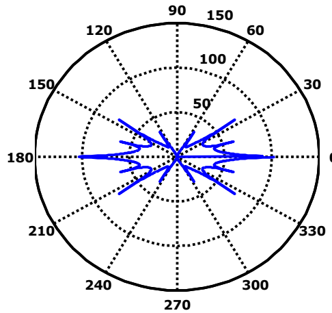
Figure 5: Variation of R(\theta, \phi) for 4 \times 4 rectangular microstrip array configuration
