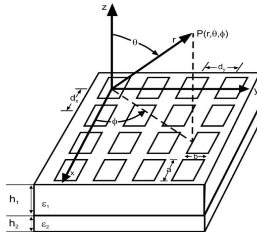
Figure 2: Geometry and coordinate system of 4 \times 4 array microstrip rectangular patch antenna
